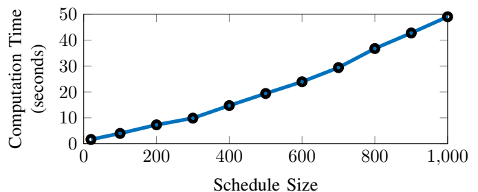
Fig. 6. The computation time for verifying the worst-case safety of schedules with different sizes. We test on 11 different sets of schedules with sizes from 20 to 1000. The data points demonstrate the O(n^2) computational complexity.
